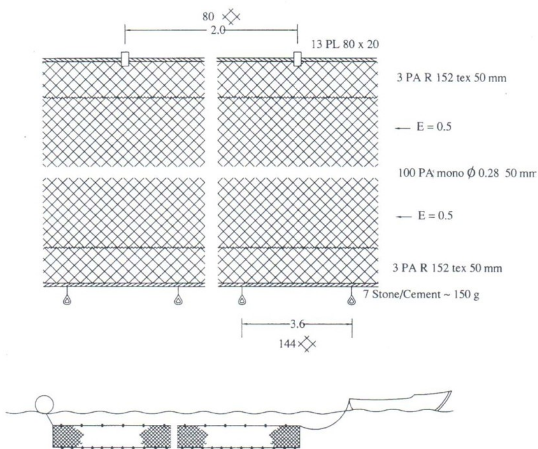
Fig. 9. Chokla jal (Surface drift net) operated in Gujarat
